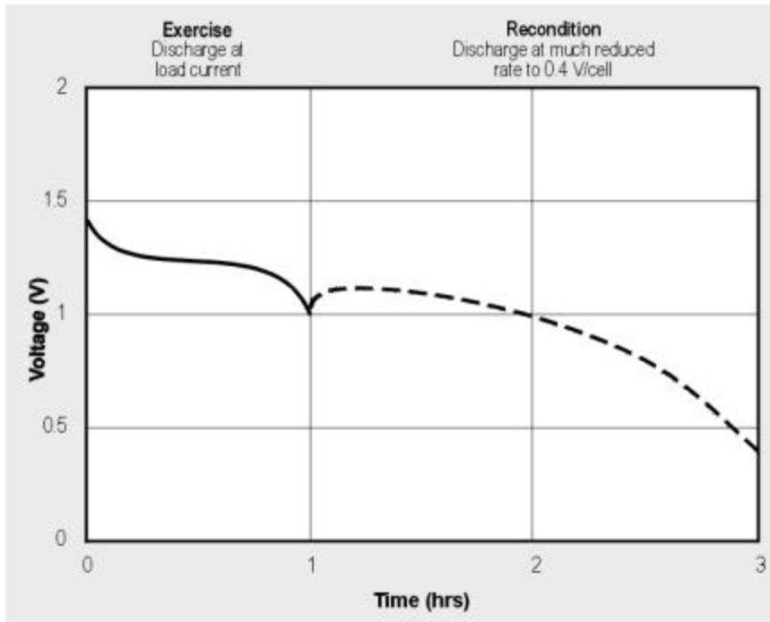
Figure 2: Exercising and reconditioning batteries on a Cadex battery analyzer. If no exercise is applied to a NiCd for three months or more, exercise may no longer be effective in restoring a battery and reconditioning is required. Recondition is a slow, deep discharge to 0.4V/cell.
